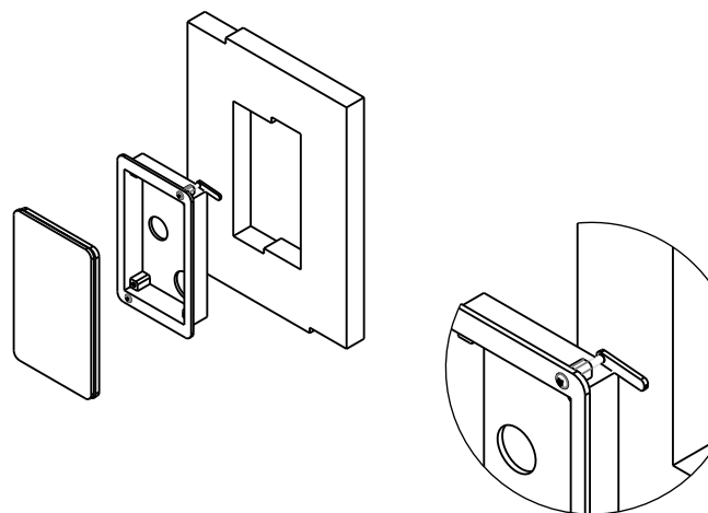
DIAGRAM 9: SL2 MOUNTING
