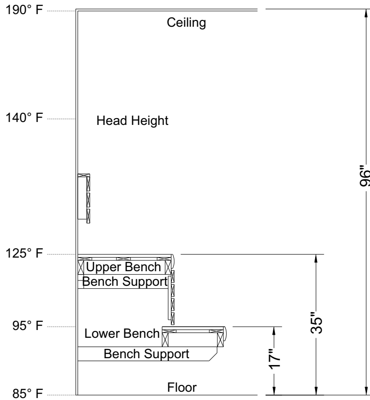
DIAGRAM 11: ROOM TEMPERATURES
