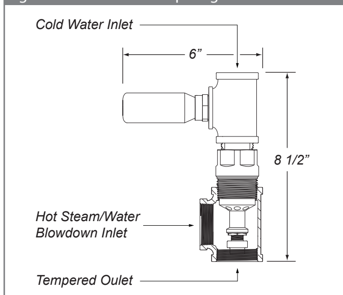
Figure 1 - Blowdown Tempering Valve
