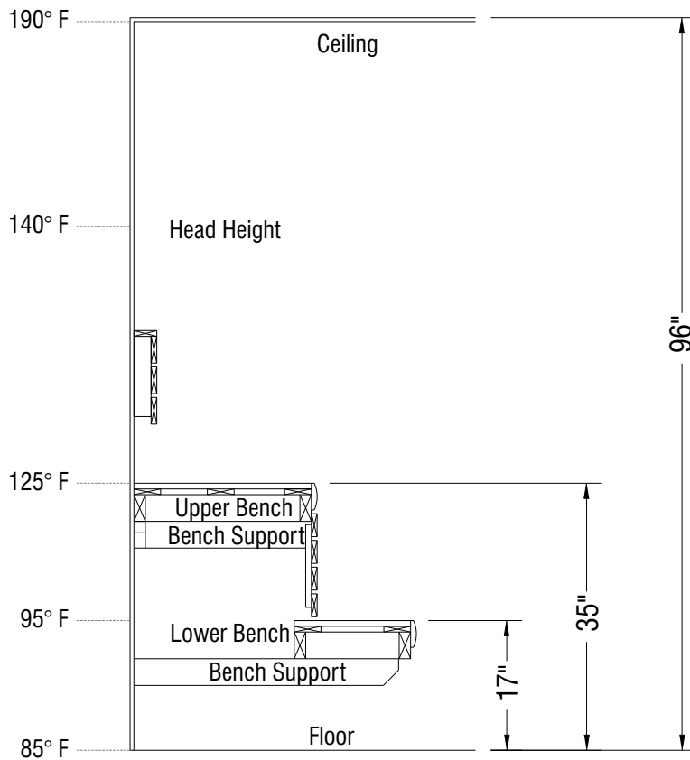
DIAGRAM 10: ROOM TEMPERATURES
