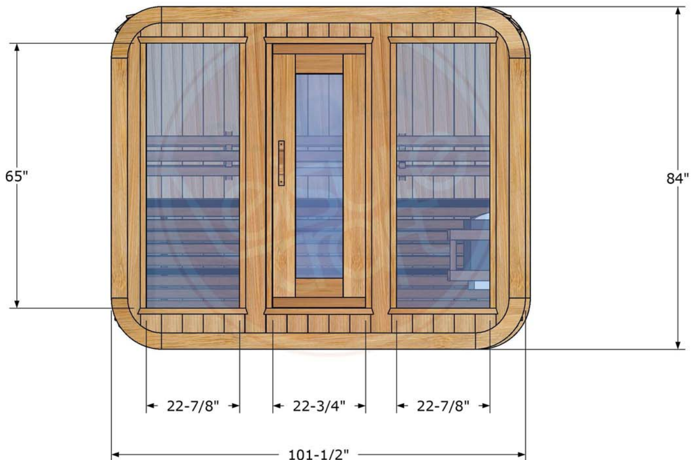
Front View
